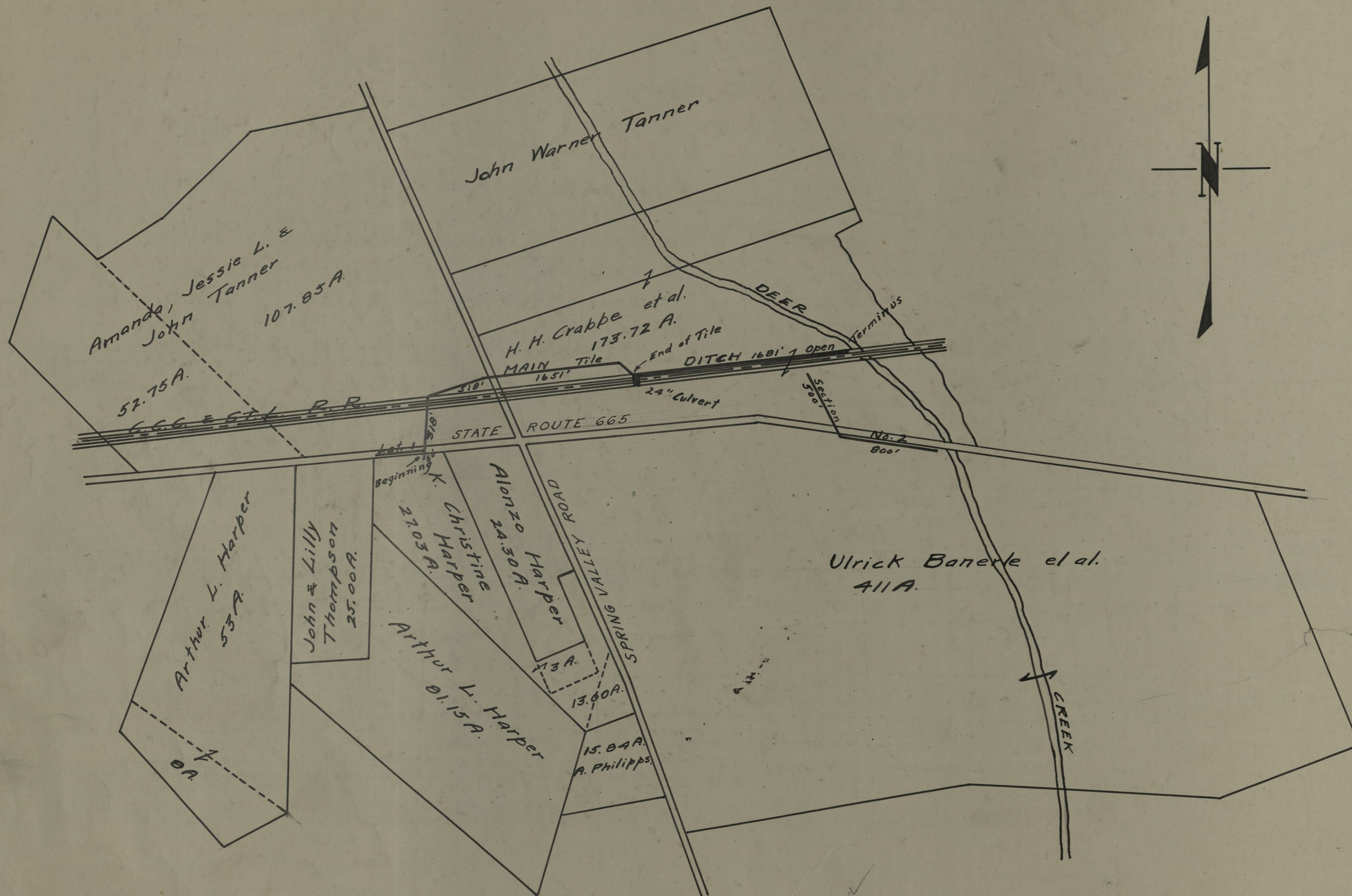
DC-WS CRABBE DITCH. UNION TOWNSHIP, MADISON COUNTY, OHIO. SCALE: 1" = 40 POLES. 1929.
