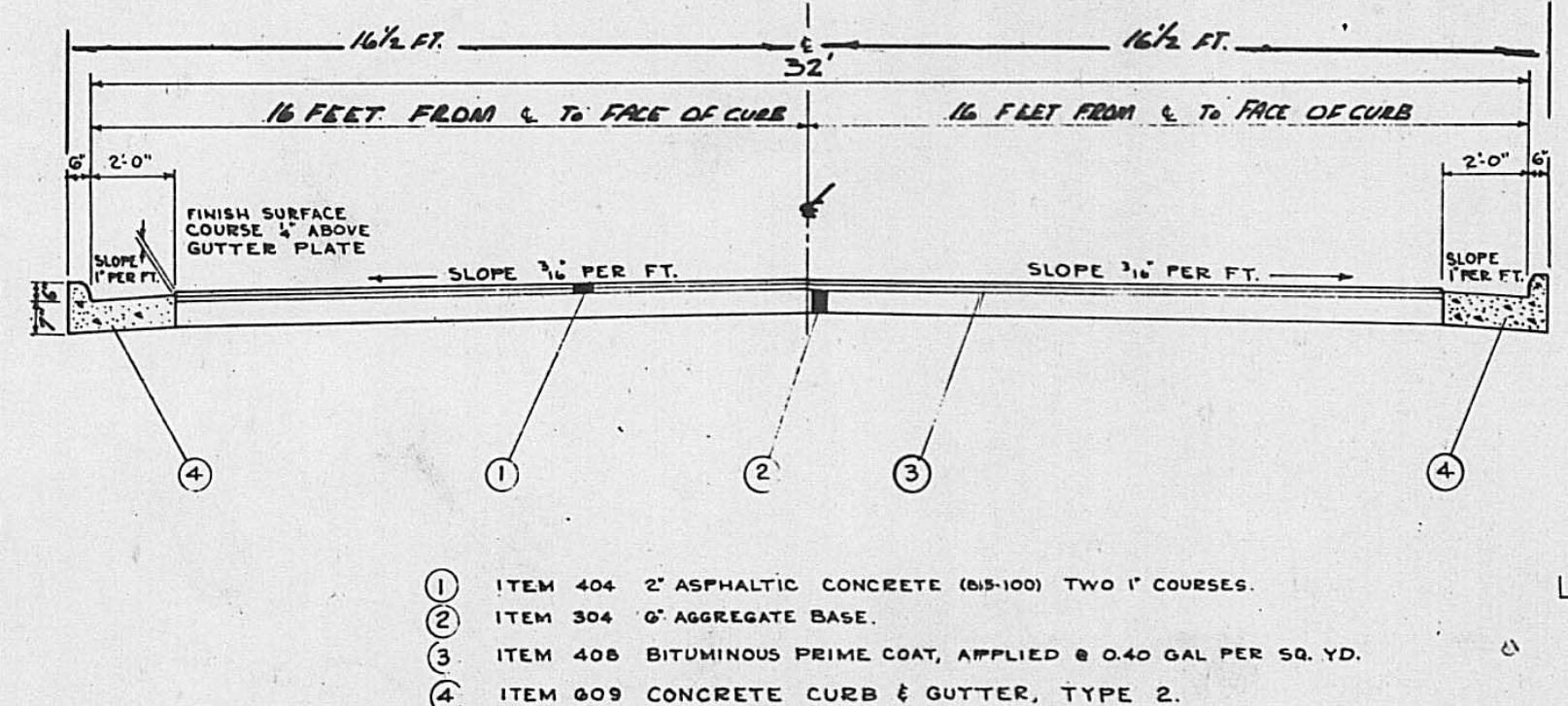
TYPICAL CROSS-SECTION
