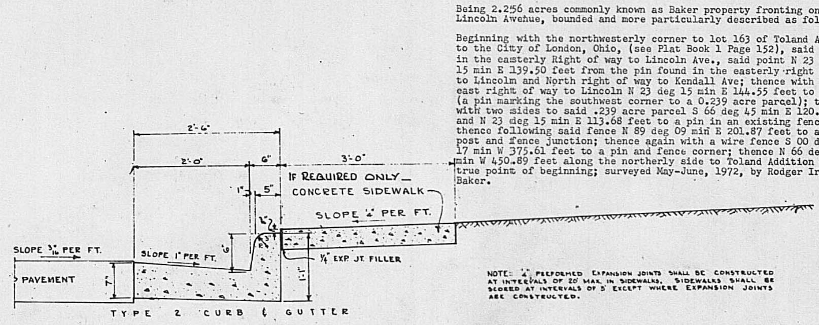
TYPICAL CROSS-SECTION
