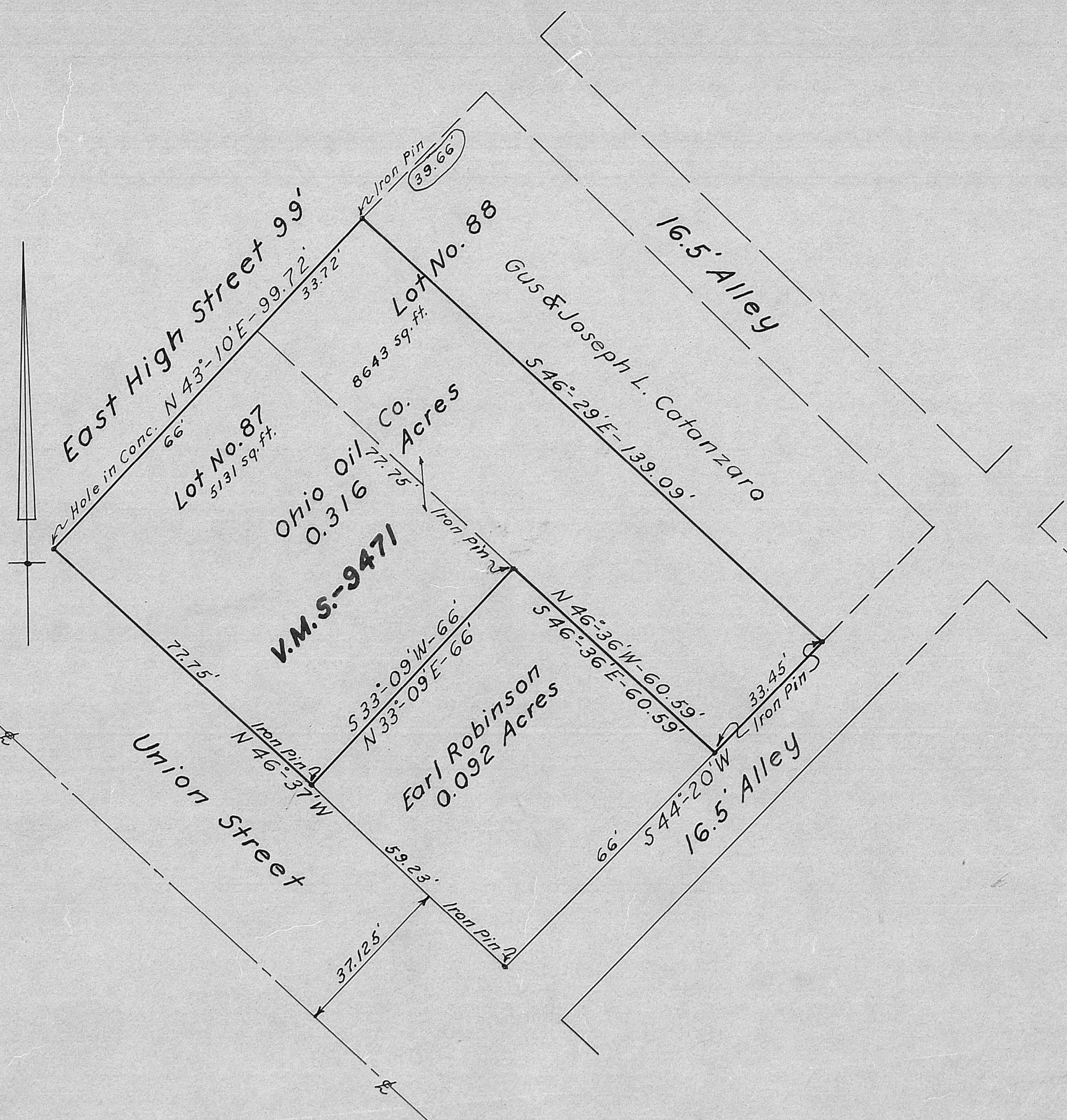
Parts of Lots No.'s 87 & 88 in the City of London, Ohio, surveyed for the Ohio Oil Company—1961
