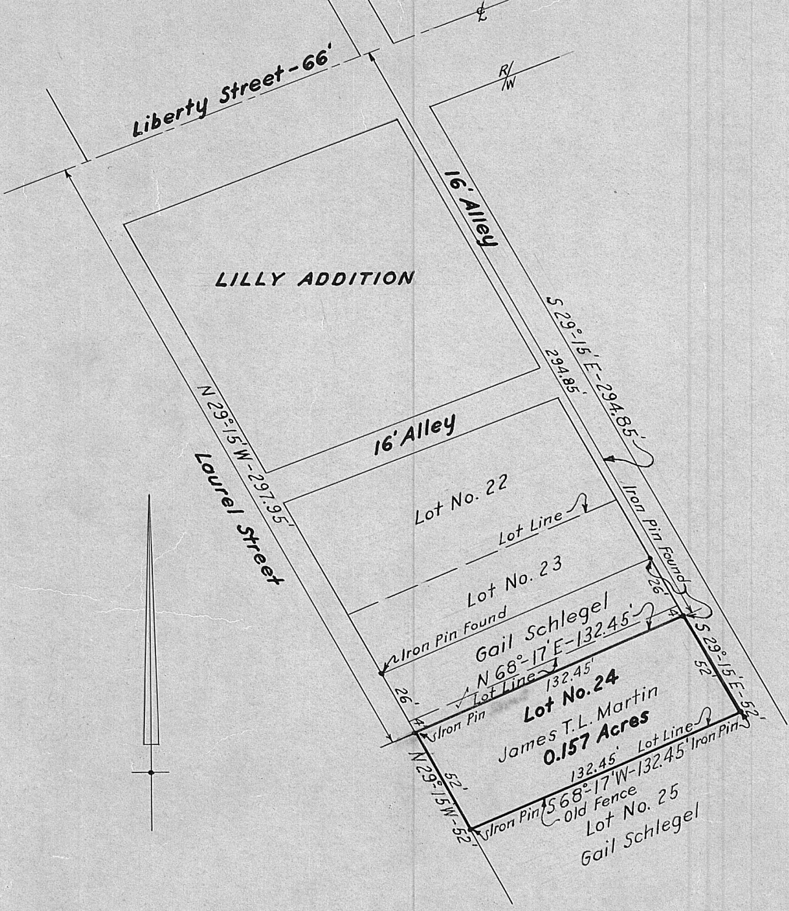
Revised Plat of parcel of land in London, Ohio, surveyed for James T.L. Martin, being part of Lot No. 24 of Lilly Addition - 1964.
