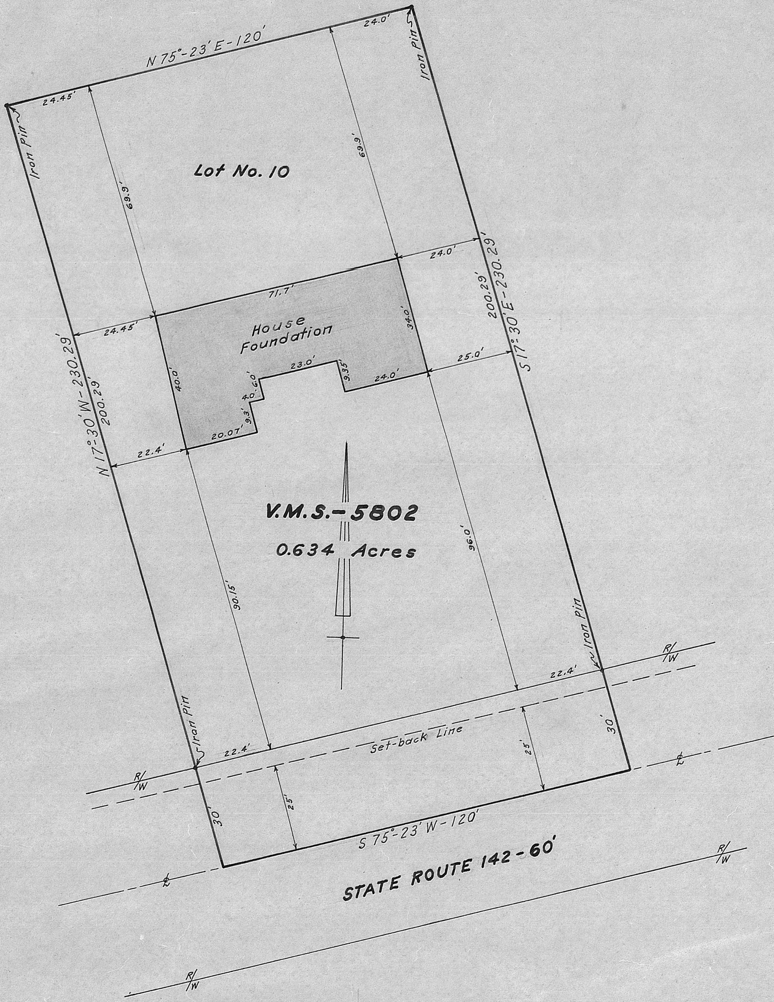
Plat of Lot No. 10 of Van Horn Construction Co. Subdivision, London Ohio, showing foundation for house construction-1966
