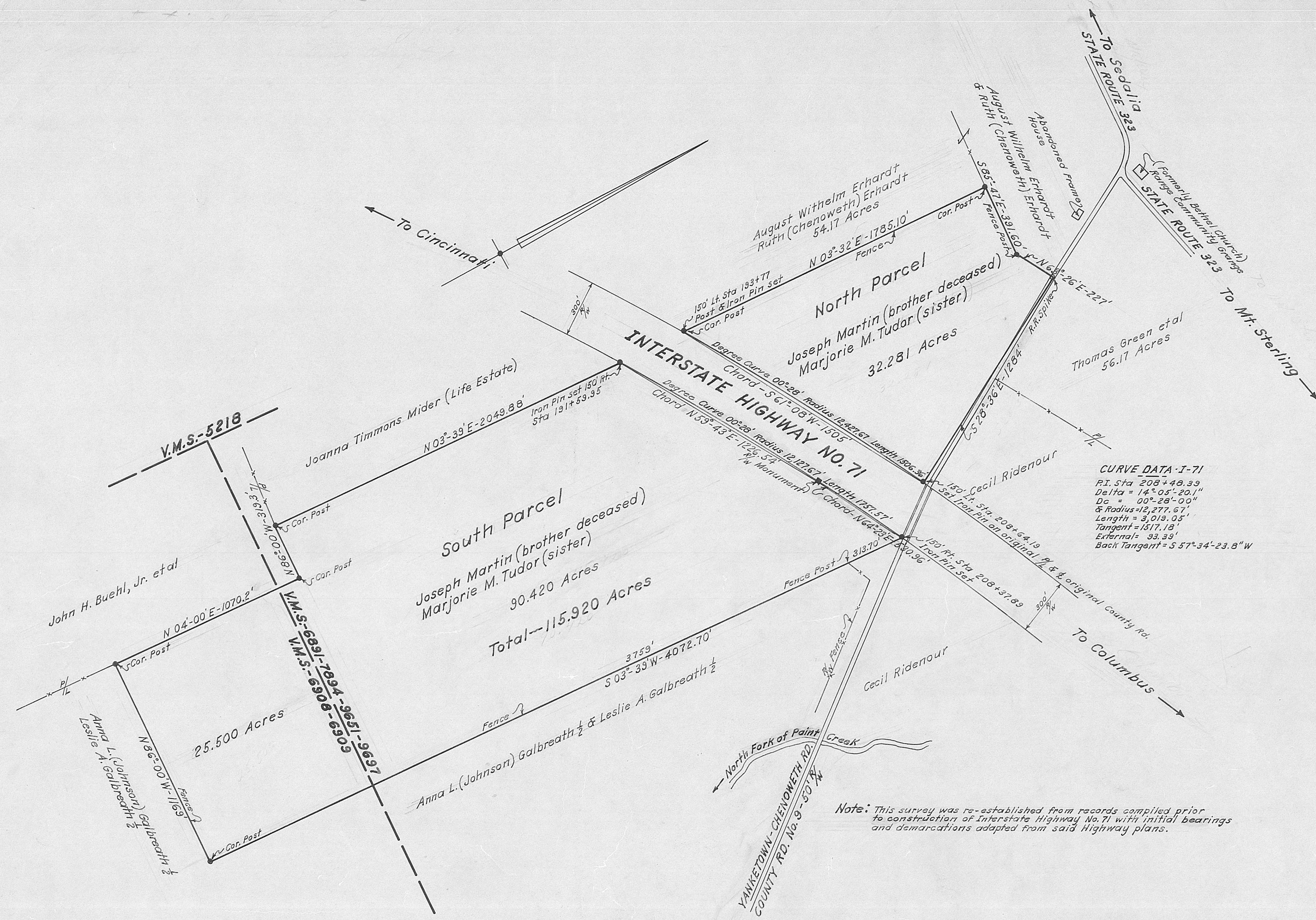
Property survey in Range Township, Madison County, Ohio, of "The Martin Farm", surveyed for Roscoe G. Hornbeck - Atty. - April, 1967
